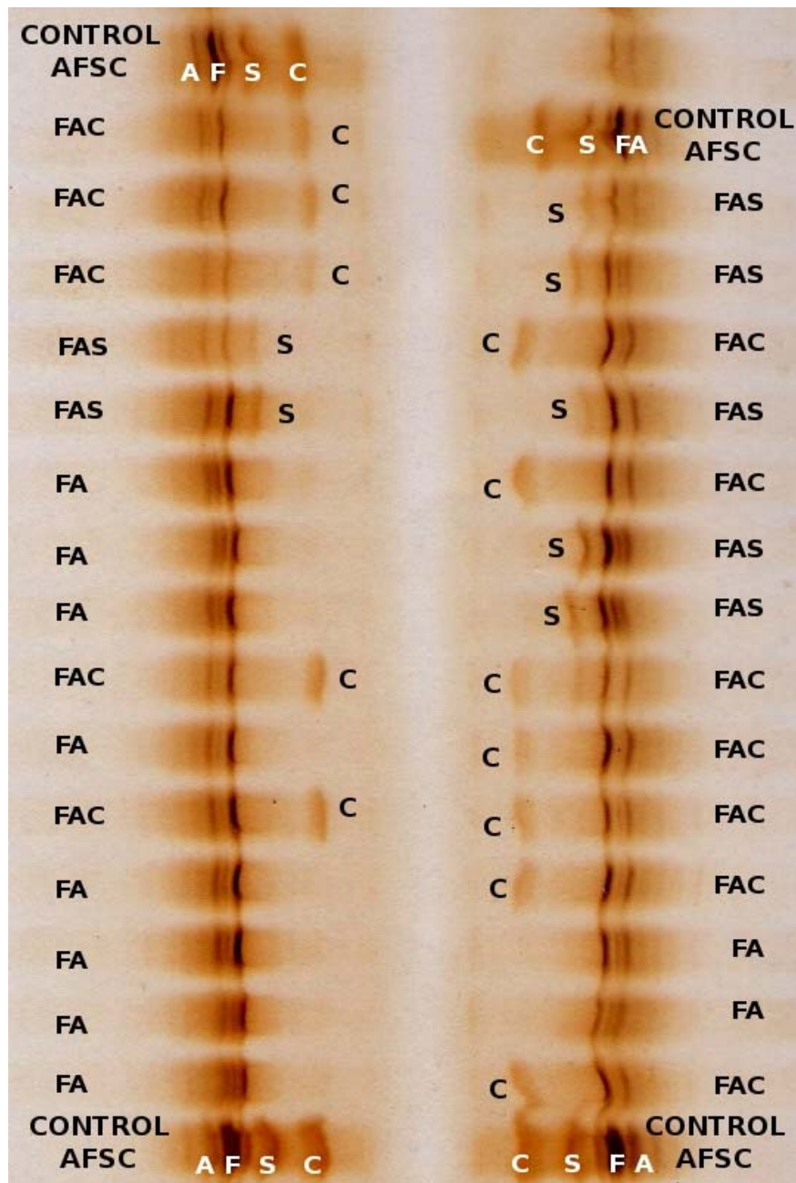
Graph 1. Hemoglobin isoelectric focusing electrophoresis
