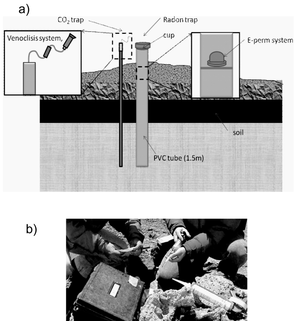
FIGURE 3. a) Example of radon and CO 2 in soil station deployment, used in this study. b) collecting data.
