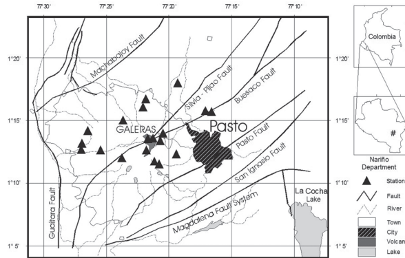
FIGURE 1. Location of the Galeras volcanic complex in the Nariño department, Colombia. Triangles represent the seismicological stations used in this study.
