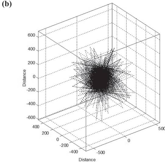
FIGURE 3. Monte Carlo simulation of the volume sampled in the single scattering process. For the simulation, an arbitrary coordinate system centered at (0,0,0) km was chosen, with an hypocenter (F1) located at (-200,-200, 0) km and one station (F2) at (200,200,0) km. A lapse time of 100 s and a velocity of 3.0 km/s were considered. (a) Horizontal projection of the Monte Carlo simulation. (b) 3D perspective of the Monte Carlo simulation.
