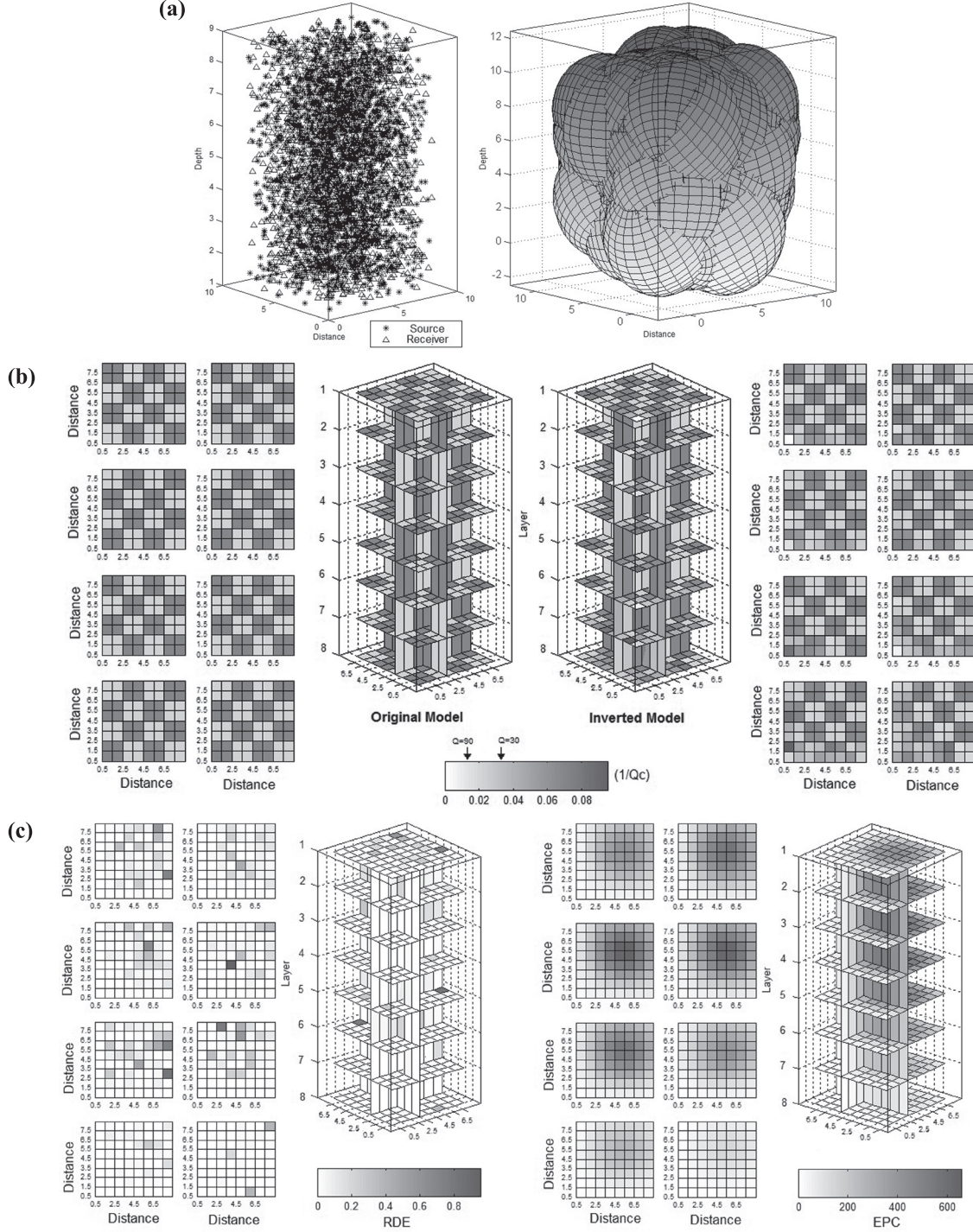
FIGURE 6. Synthetic test in a 3D attenuation model of 8 \times 8 \times 8 blocks. (a) Distribution of 2000 random pairs of foci (left) and ellipsoids related to volume sampled in the simple scattering process (right). (b) Original and inverted attenuation models with Q_c values of 30 and 90. (c) Spatial distribution of RDE and EPC.
