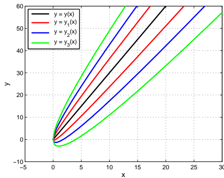
Figure 8. \lambda_0 = 1.0, \lambda_1 = 2.0 .
