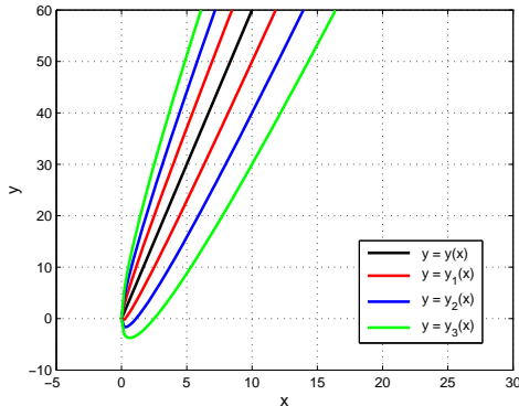
Figure 9. \lambda_0 = 1.0, \lambda_1 = 5.0 .
