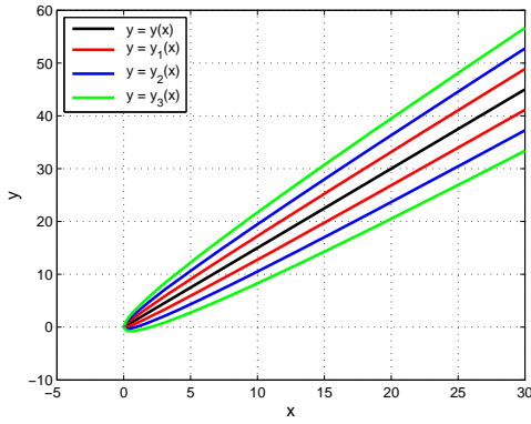
Figure 2. \lambda_0 = 2.0, \lambda_1 = 1.0.
