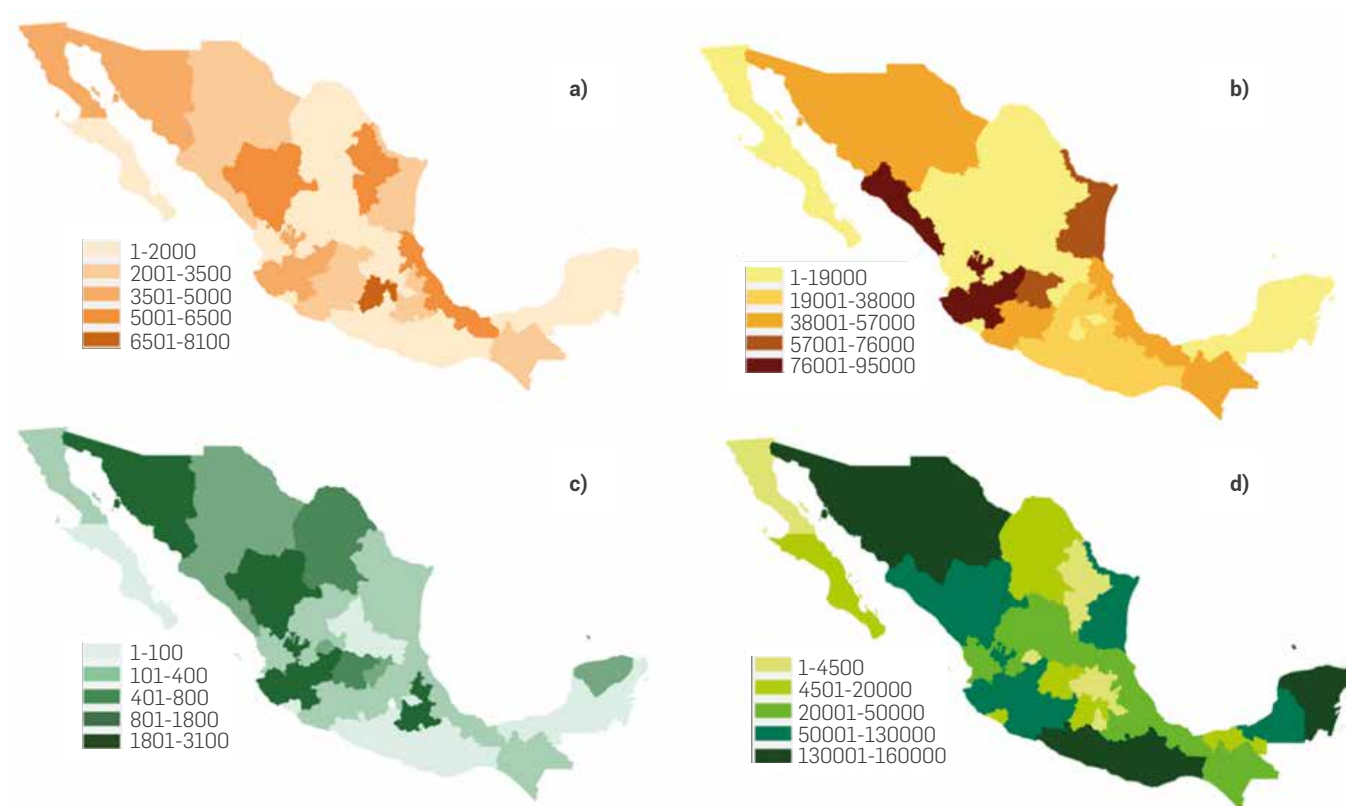
Figure 4. Biomass resources (TJ/year) from different sources in Mexico. a) Urban waste. b) Agricultural and forestry waste. c) Livestock residues. d) Sustainable logging. Source: Adapted from [6], [7].
