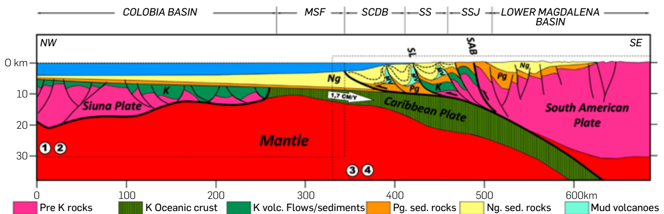
Figure 3. Crustal section through the Caribbean Plate and the NWCSA (See location on map in Figure 2 ). Note the thickness variations of the Caribbean Plate along the Colombia Basin and the volcanic-sedimentary (K) sequences that cover it towards the NW (especially in the area of the Siuna Plate), the thin sedimentary sequence of the Paleogene (Pg), as well as the increase in thickness of the sedimentary sequences accumulated from the mid-Miocene (Ng) towards the SW, in the area of the Magdalena Submarine Fan (MSF) and the Southern Caribbean Deformed Belt (SCDB), up to the Sinu Lineament (SL). The area of the SCDB and the Serranía de San Jacinto (SS) present complex deformation, combined with mud volcanism (MV), extended to the limit with the South American Plate (SAB), product of the convergence with the Caribbean Plate. The numbers indicate the reference selected to build the section in the area limited by the dotted line polygons: 1) Ewing [46]; 2) Romito and Mann [47]; 3) Bernal-Olaya [52]. 4) López-Ramos [53]. The convergence rate of the Caribbean Plate is taken from Mora-Paéz [56].
