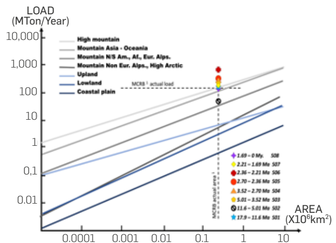
Figure 23. Global load relationship (vertical axis) vs. river basin area (horizontal axis) in different topographic areas [5] and the position occupied in this relationship by the current area and load of the Magdalena - Cauca River Basins -MCRB - according to the values calculated in previous works [25]. Note the variation in the sedimentary load for each sedimentary sequence (S01 to S08), estimated from the analysis of accumulated sedimentary volumes in the CB, SCDB and MSF during the last 18 My.
