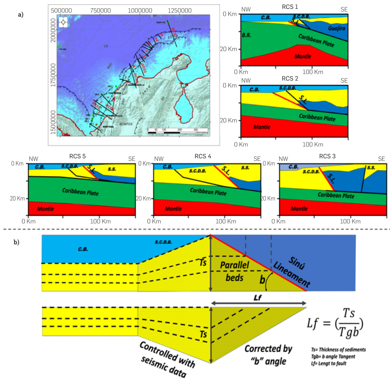
Figure 11. Regional geological sections used to estimate the angle b=25^\circ of the Sinu lineament (L.S. panel a) and location map of Regional cross sections (RCS) 1 to 4 [34], [36]; RCS 5 [131]. Below (b), explanatory diagram of thickness estimation from the limit of the Colombia Basin to the dipping fault between the recent and old deformed belts. The thicknesses of the sequences were taken from the engages of each sequence interpreted in the Colombia Basin (C.B.), while in the Southern Caribbean Deformed Belt (SCDB) and the Serranía del Sinú (S.S.), it was controlled with 2D regional seismic lines (sections 1 to 15 in the map). The thicknesses in the recumbent block of the S.L. were considered parallel to its intersection with the fault plane and were corrected to surface considering the b angle.
