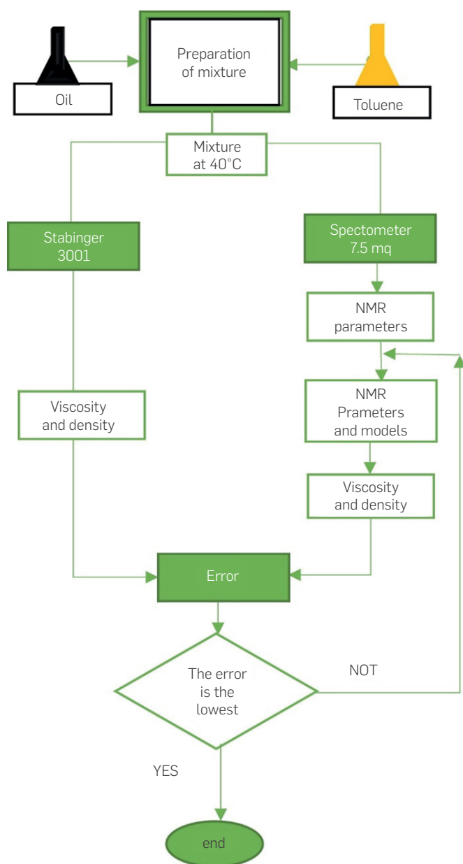
Figure 1. Workflow to evaluate NMR model and to determine the density and viscosity values
