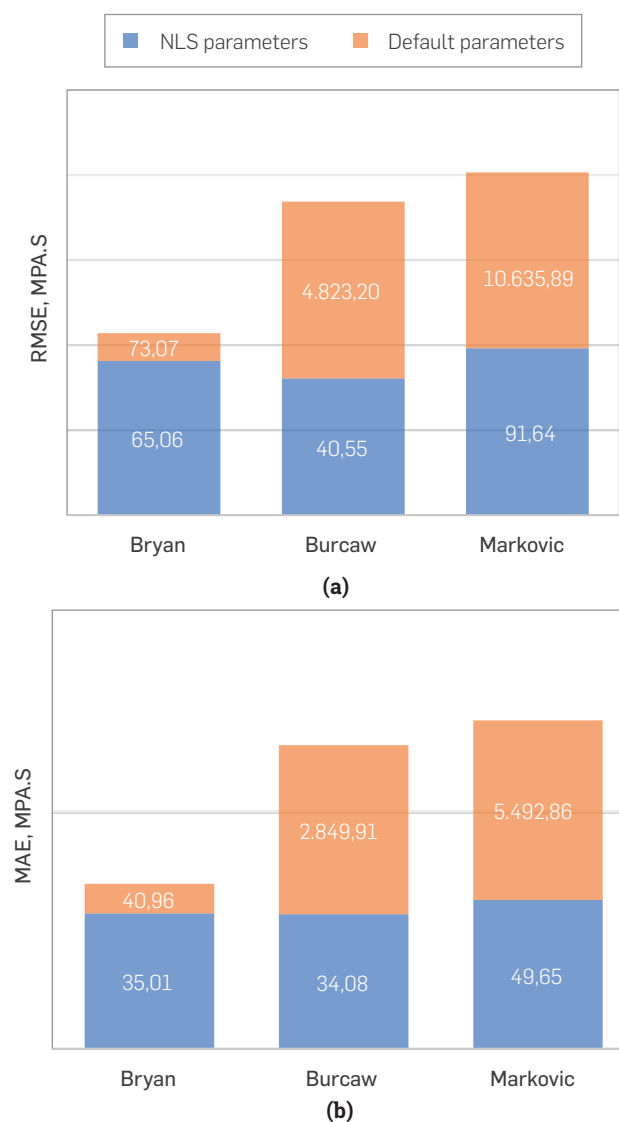
Figure 7. Compared (a), Root-MSE (b) and MAE of NMR model predictions for using three model configurations. Bryan (2003), Burcaw (2007) and Markovic (2020)
