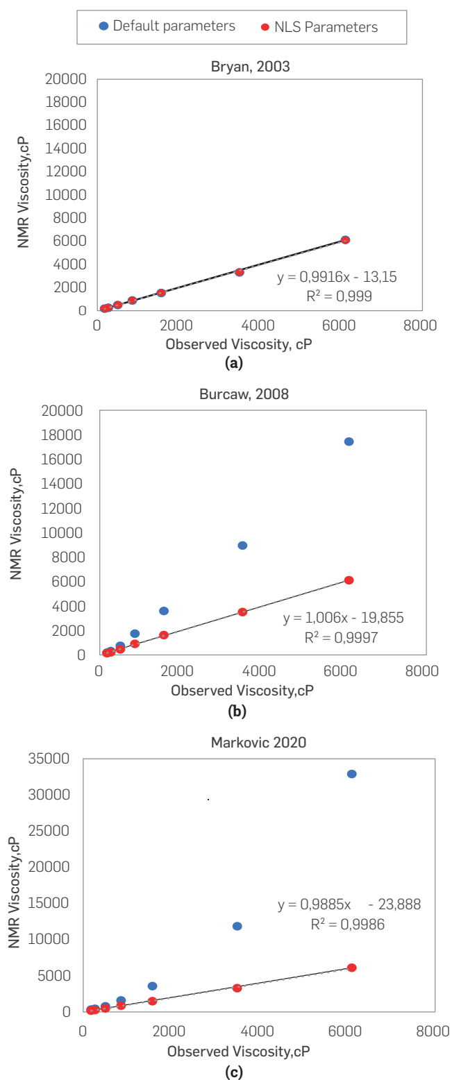
Figure 6. Rheological viscosities compared to NMR viscosities of 7 samples. Solid black line (1:1) presents a perfect prediction for all models.
