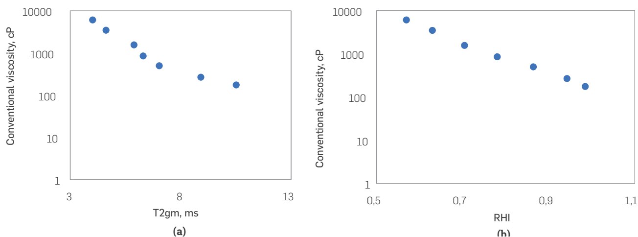
Figure 4. Relationship of the NMR parameters (a) Viscosity vs T2gm (b) Viscosity vs RHI
