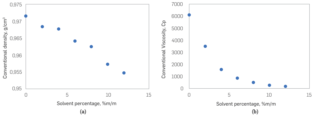
Figure 2. Mixtures density and viscosity relation with the toluene concentration.
