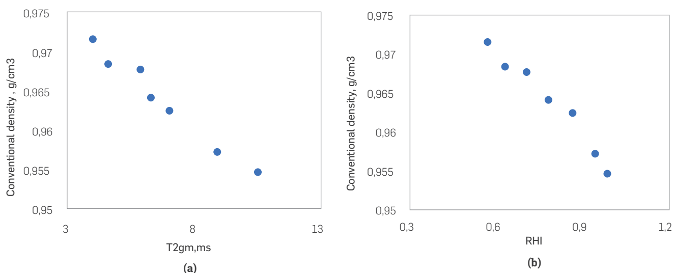
Figure 5. Density relationship with NMR parameters. (a) Density vs T2gm (b) Density vs RHI
