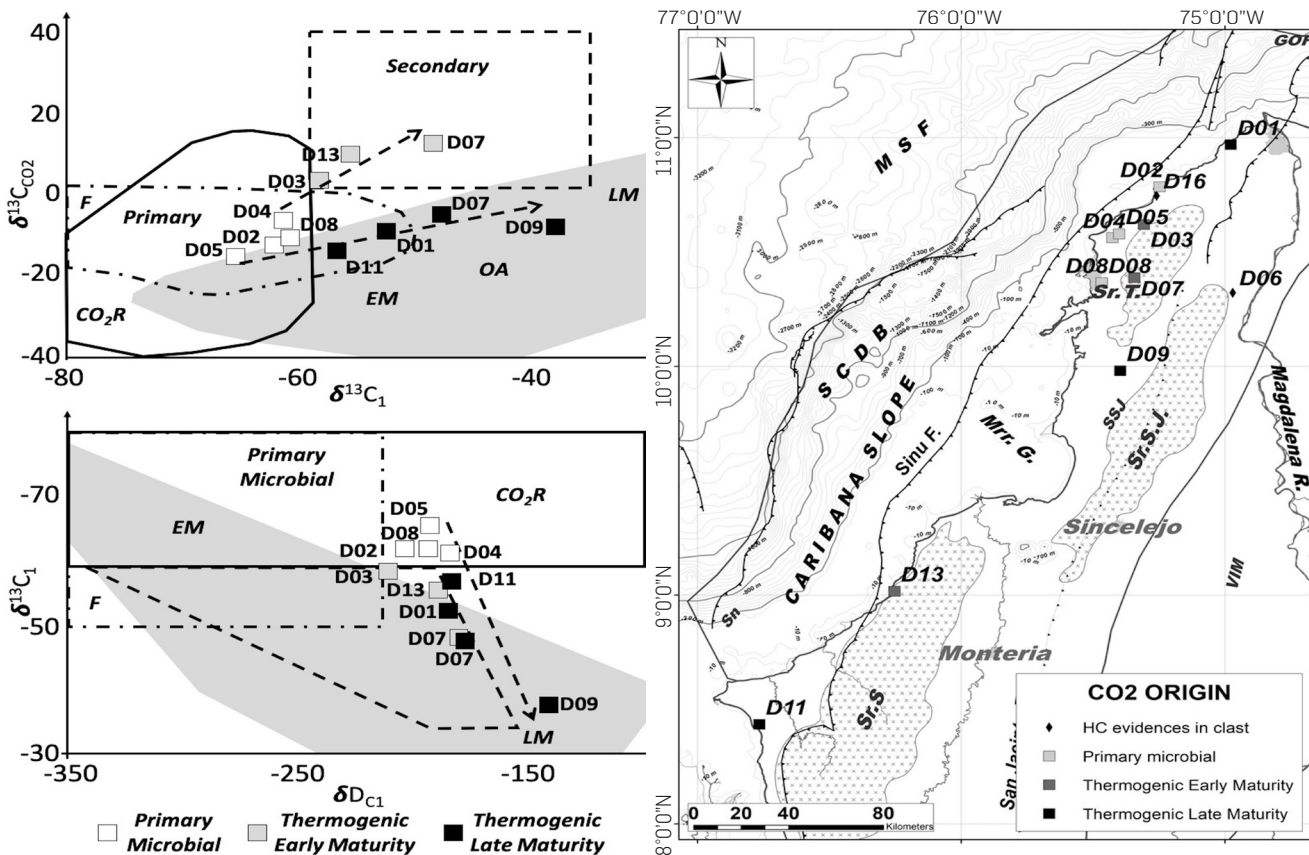
Figure 12. Left upper diagram \delta^{13}C_1 vs \delta^{13}C_{CO_2} , bottom diagram \delta^{13}C_1 vs \delta D_{C1} , and their relationship to CO 2 generation (Milkov and Etiope, 2018). Primary microbial natural gas, generated by the activity on an organic precursor of the source rock by: F= Fermentation or by CO 2 ; R= CO 2 reduction. Thermogenic natural gas of different stages of maturity: EM= early maturity gas; OA= gases associated with an oil; LM= gases associated with a late maturity. Volcanoes: 1= La Laguna; 2= Las Palomas; 3= Santa Catalina; 4= Yerbabuena; 5= El Reposo; 7= Cañaveral; 8= El Rodeo; 9= Flamenco; 11= Virgen del Cobre; 13= Puerto Escondido. Right, distribution map of mud volcanoes and their classification according to CO 2 isotopic origin analysis. Data sources are recorded in Table 6 for the mud volcanoes sampled during this work.
