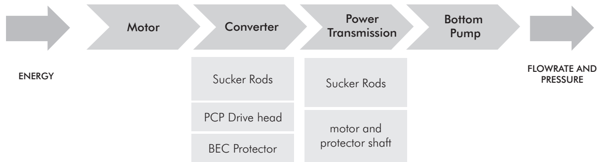
Figure 2. Power transfer in artificial lift systems
