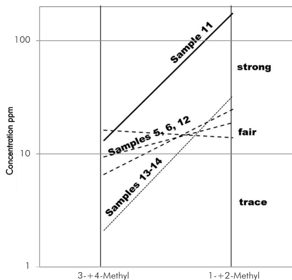
Figure 6. Graphic of concentration in ppm of 3- + 4- methyldiamantenes and 1- + 2-methyldiamantenes. Note that the samples recovered to the south of the Tumaco high show less concentrations in diamantoids in comparison with the samples analyzed to the North.
