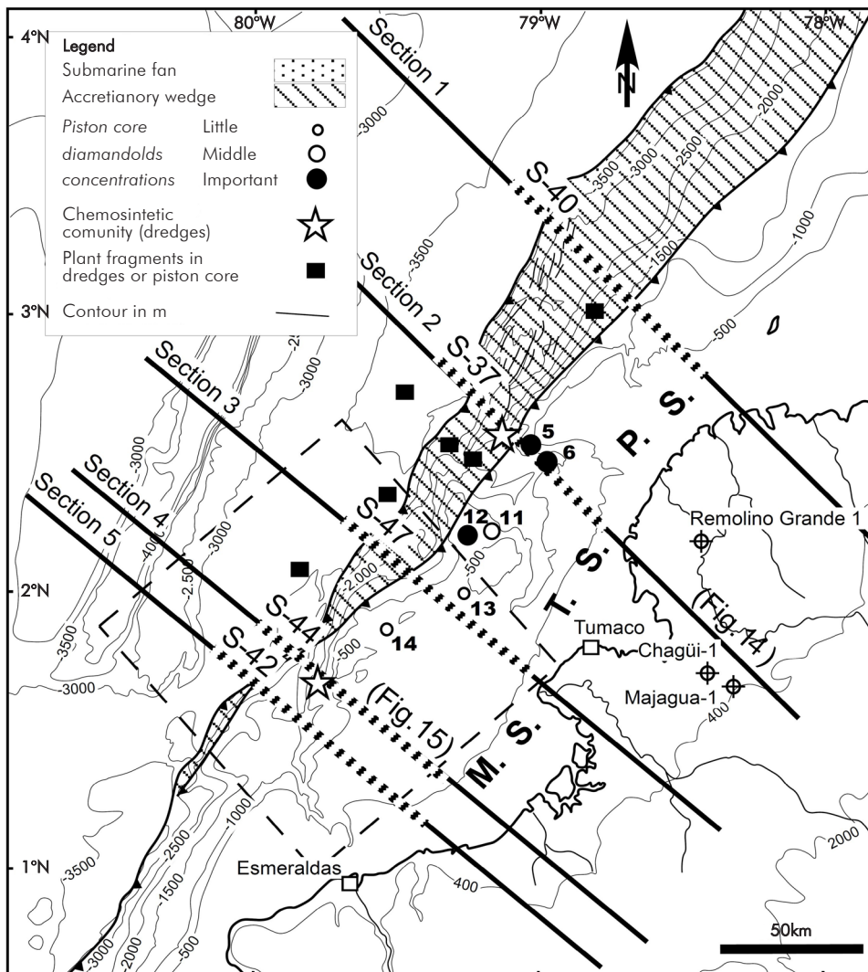
Figure 7. Location of regional cross sections (lines 1-5) used to construct 2D TTI arr models along the NESC margin subduction zone. Line segments with diagonal white pattern indicate the location of multichannel seismic reflection profiles (S-37, S-40, S-42, S-44 and S-47) used during the construction of the structural geometry of each section (modified from Marcaillou et al. 2008; Collot et al. 2009). TOC values in the Tumaco basin was obtained from the exploratory wells drilled in the Tumaco basin described by Cediél et al. (2009). Black squares show the location of the piston cores and dredges with fragments of plants carried from the forearc zone (Collot et al., 2005). The dashed line box shows the location of the ESMERALDAS 3D seismic refraction survey (modified from García – Cano et al. 2014). Piston core (circles) and dredges samples (white stars) are the same described in the Figure 4. The Manglares (MS), Tumaco (TS) and Patía (PS) thermal segments correspond to the definition of Marcaillou et al. (2008).
