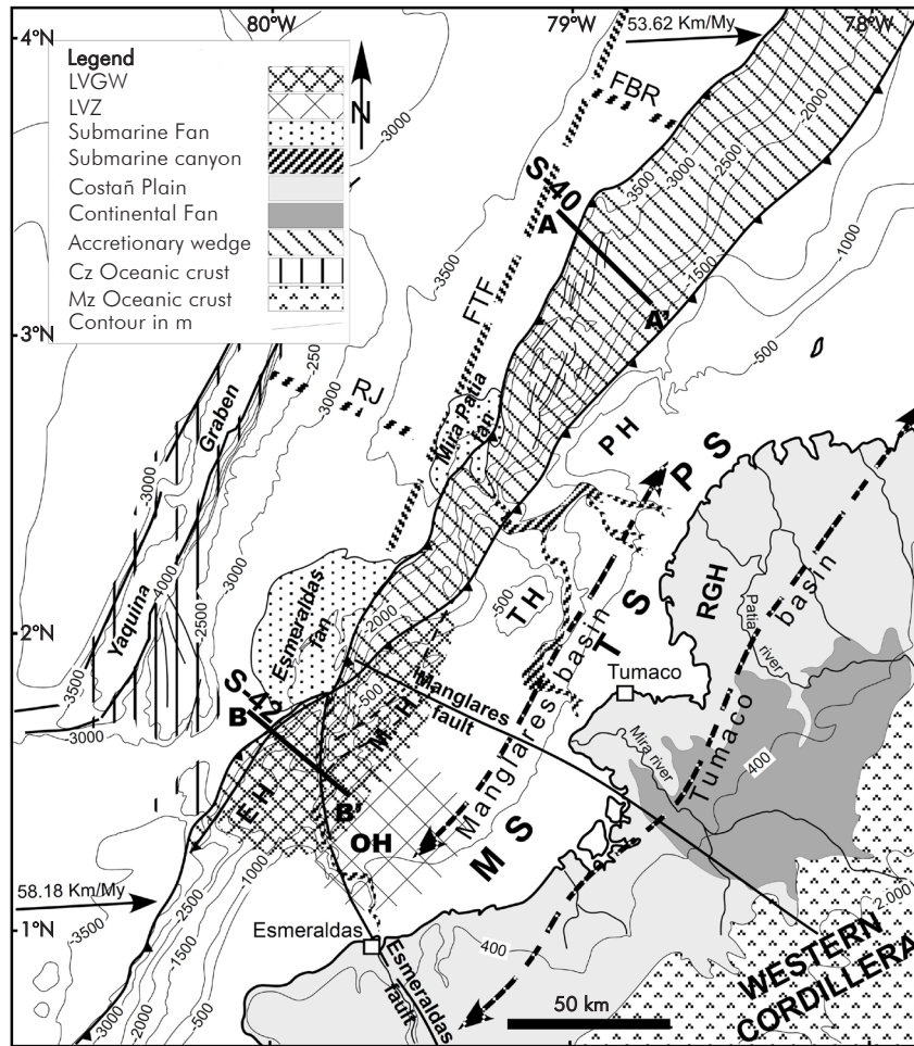
Figure 2. Map with the main morphologic and tectonic features observed along the NESZ. The margin is bisected by several submarine canyons (Esmeraldas, Mira and Patia), that provide sediments to associated, distal submarine fans. The Tumaco and Manglares basins are oriented parallel to the subduction zone, divided by the Remolino Grande High (RGH), outlining a double forearc basin system. A discontinuous chain of structural highs known as Esmeraldas (EH), Manglares (MH), Tumaco (TH) and Patia (PH) outline the seaward border of the NESZ margin double forearc basin. To the west of these structural highs the accretionary wedge increases in width toward the North, suggesting a transition from tectonic erosion in the south to a regime of tectonic accretion in the north (modified from Marcaillou et al. 2006 and Marcaillou et al. 2008). Note that the overriding plate is segmented by the Manglares and Esmeraldas faults that divide the thermal structure of the NESZ margin into the Manglares (MS), Tumaco (TS) and Patia (PS) segments (modified from Marcaillou et al. 2008). In the Manglares segment seismic refraction experiments have detected altered basement zones known as the Low Velocity Zone (LVZ) and Low Velocity Gradient Wedge (LVGW) (modified from García – Cano et al. 2014 and Collot et al. 2008). To the west of the Manglares segment, the basement of the Nazca Plate is extensively exposed at the sea floor along the Yaquina Graben walls. In addition, seamounts are faulted by the Fossil Transform Fault (FTF) and Ridge Jump (RJ) structures. (Hardy, 1991). Heavy lines (S-40 and S-42) indicate lines of cross sections shown in the Figure 3.
