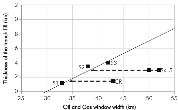
Figure 13. Thickness of the trench fill sediments undergoing subduction versus the oil and gas window width along the subduction zone of the five sections modeled in the NESM margin (Section 1: S1; Section 2: S2; Section 3: S3, Section 4: S4, Section 5: S5). For comparison purposes, data from the Costa Rica margin (CR) from Lutz et al (2004) is plotted. Note that the sections S1 to S3 (Patía and Tumaco segments) define a linear relationship showing that the sediment thickness in subduction zones constrains the width of the oil and gas windows, while sections S4, S5 and CR (Manglares segment and Costa Rica margin) are not congruent with this relationship and suggest an additional mechanism to explain the enhancement of the current oil and gas windows like hydrothermal circulation in the subducting plate. x-axis label should read 'Oil and Gas window width (km)'
