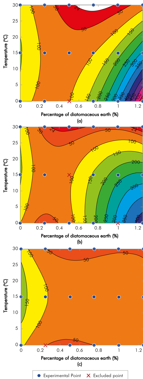
Figure 3. Contour plot for Total Contamination (mg/kg) in treated biodiesel samples: a) BE3; b) BE1 and c) BE2.
