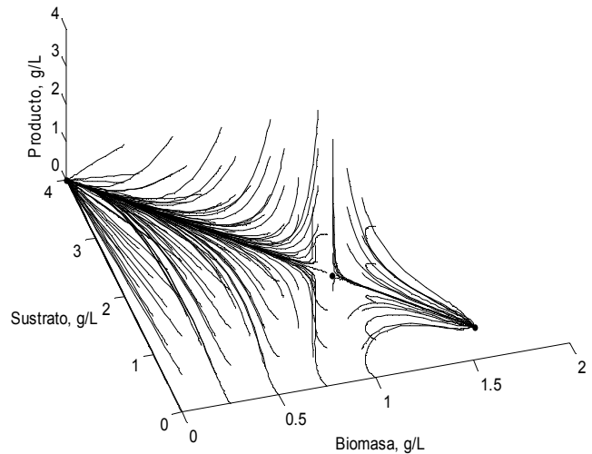
Figura 8. Plano de fase modelo Haldane Figure 8. Phase plane for the Haldane model
