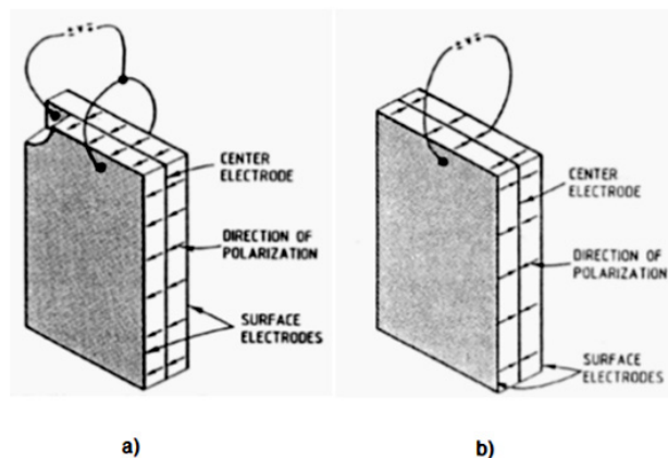
Figure 2. Bender elements: a) parallel; b) series [2]
