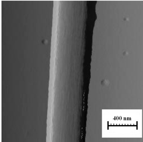
Figure 6. AFM topographic image (2 μm x 2 μm) of a PVA nanofiber.
