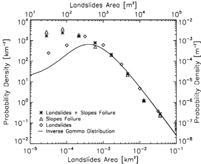
Figure 4. Comparison of the probability density of landslides according to the area of the data taken on the field and a theoretical function of the Inverse Gamma type.
