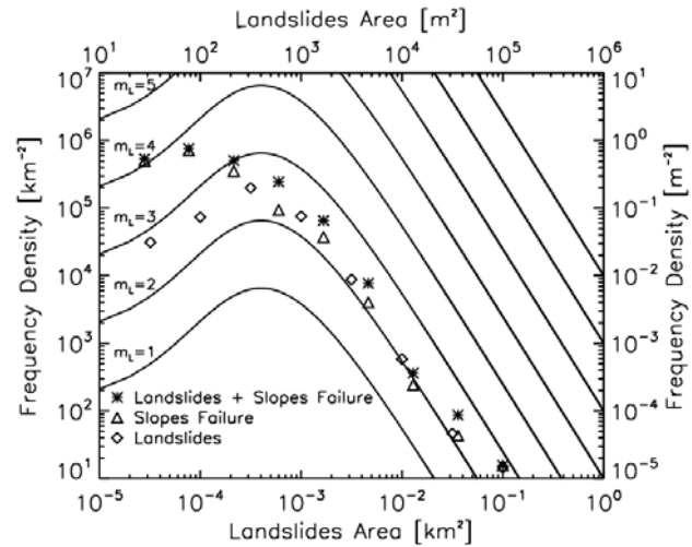
Figure 5. Theoretical and real magnitudes of the different groups of landslides of the field survey taken for this work.
