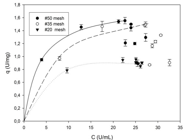
Figure 3. Adsorption isotherms of PPase-SE to lemon protopectin in CitB (10 mM, pH 5.0) at 4 – 8 °C with shaking at 150 \text{ rpm} . The concentrations of enzyme and substrate were 25 \text{ U}\cdot\text{mL}^{-1} and 20 \text{ mg}\cdot\text{mL}^{-1} , respectively. Source: The Authors
