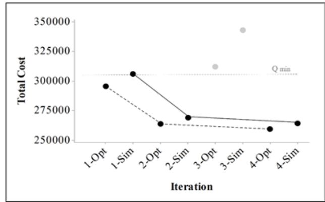
Figure 5. Obtained costs from the optimization and simulation models in each iteration for scenario two.
