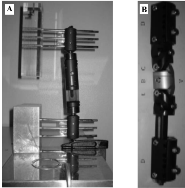
Figure 13. External fixation system used for comparing the stiffness. A) ProCallus from Orthofix (Verona, Italy). B) Dynamix DFS from Ebifex (Iowa, IA, USA). Source: [10].
