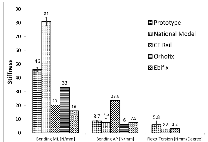
Figure 16. Stiffness under medio-lateral (ML) bending, antero-posterior (AP) bending, and flexo-torsion loading. The bars represent the standard deviations.
