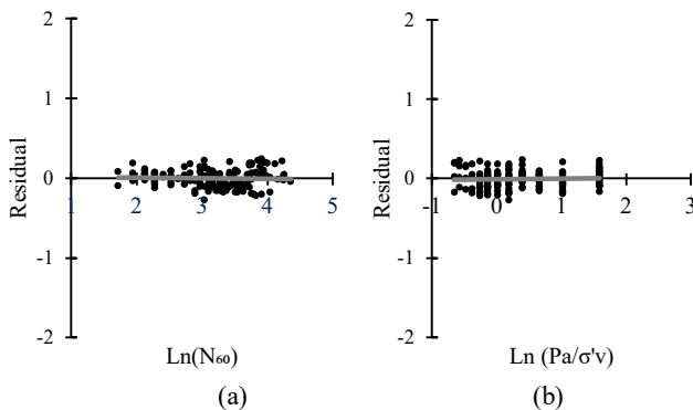
Figure 12. Residuals of the multiple linear regression model for sands. (a) residual versus \ln(N_{60}) . (b) Residual versus \ln(P_a/\sigma'_v) . Source: The authors.
