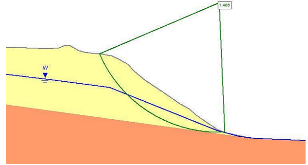
Figure 15. Profile 6 – a situation with critical groundwater Source: Author
