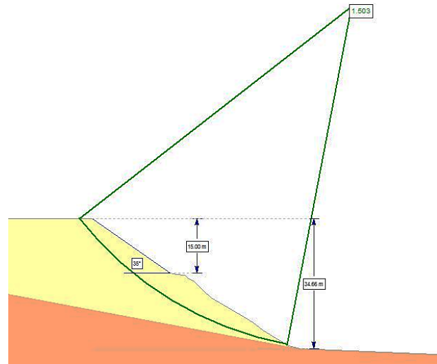
Figure 16. Profile 1 Final - normal case Source: Author
