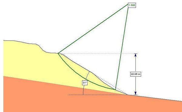
Figure 8. Profile 3 - normal case Source: Author
