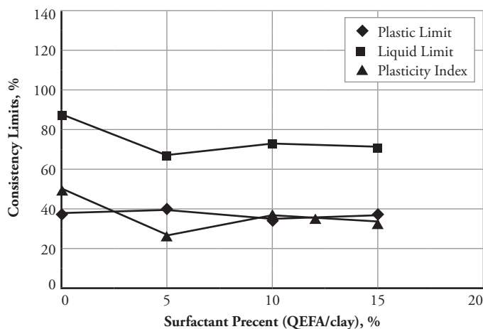
Figure 9. QEFA effect on clay's consistency limits.
