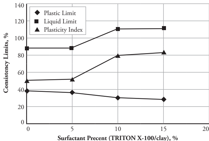
Figure 5. TRITON X-100 effect on clay's consistency limits.
