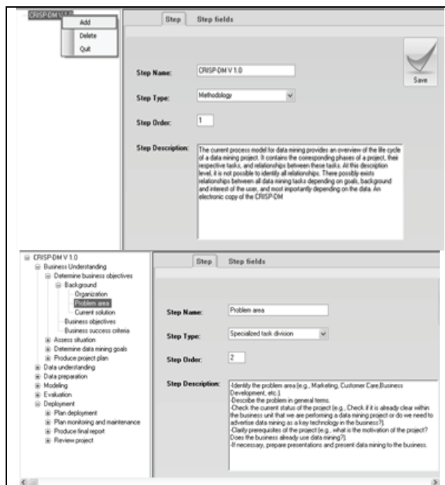
Figure 3. Steps in a process (left) and CRISP-DM in CMIN (right)
