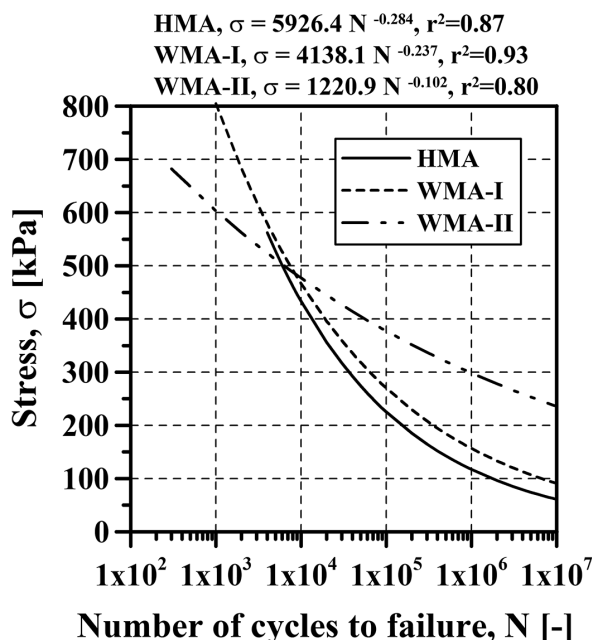
Figure 5. HMA and WMAI and II Fatigue Curves (LTOA) – Stress.
