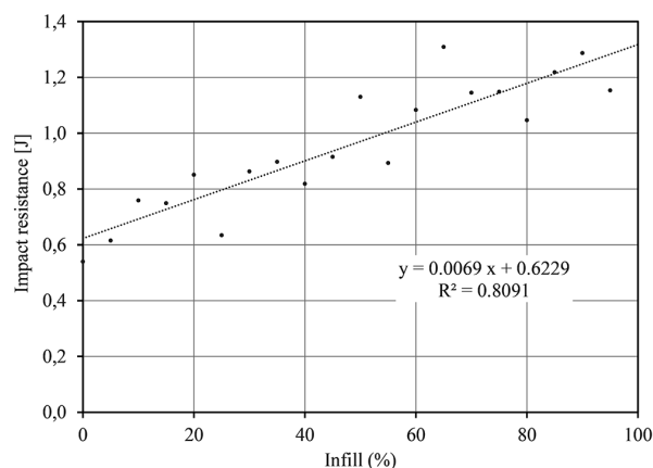
Figure 6. Impact resistance vs. infill percentage.
