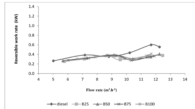
Figure 3. Reversible work rate vs. flow rate (maximum pump speed) Source: Authors
