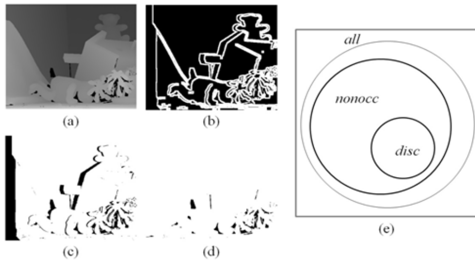
Figure 4. Illustration of error criteria (white areas) using the Teddy stereo image, (a) ground-truth disparity map using gray levels, (b) disc criterion in white color, (c) nonocc criterion in white color, (d) all criterion in white color, (e) generalisation of conventional error criteria using Venn diagram
