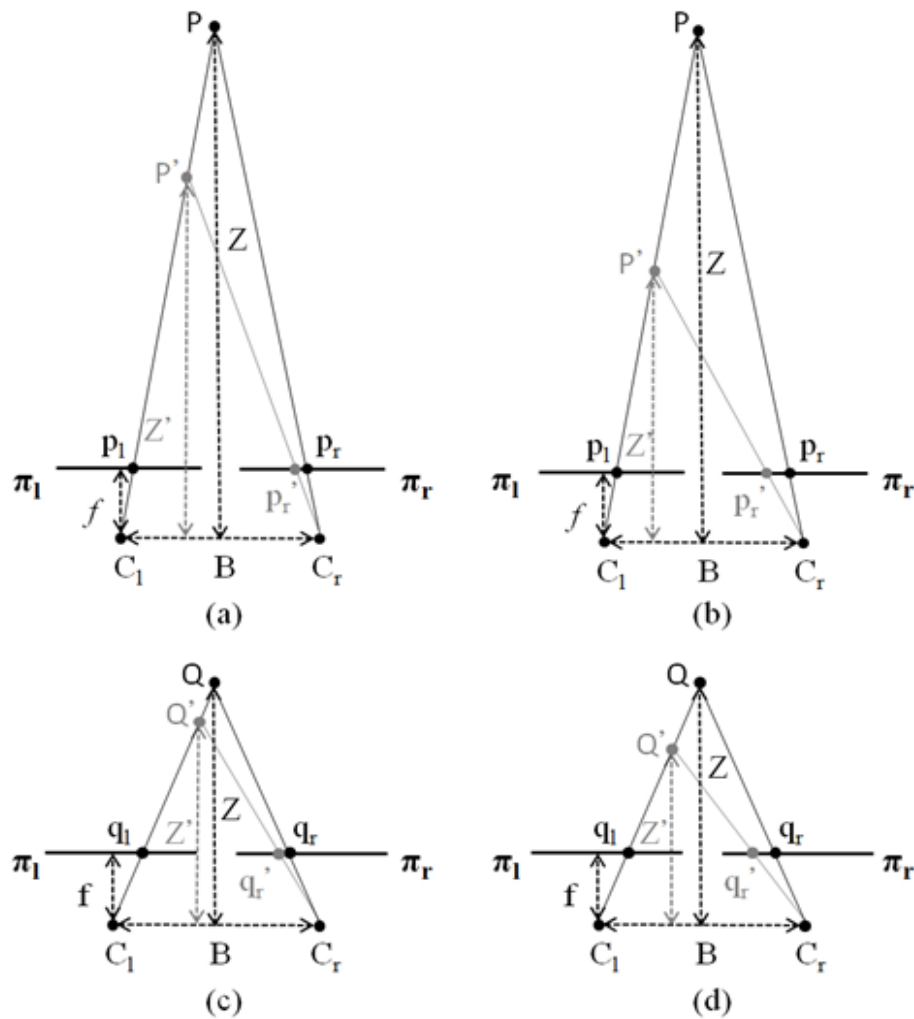
Figure 2. Disparity estimation errors vs. triangulation errors: (a) small estimation errors of a farther point, (b) larger estimation error of a farther point, (c) small estimation error of a close point, (d) large estimation error of a close point
