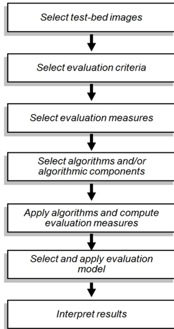
Figure 1. Evaluation methodology
