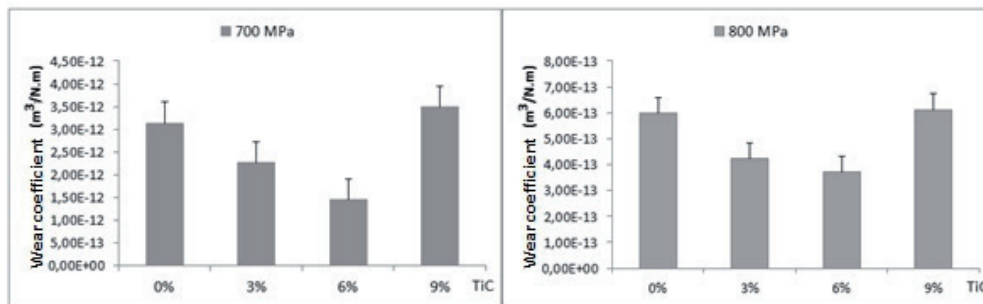
Figure 8. Wear coefficient of sintered compacted at 700 and 800 MPa.
