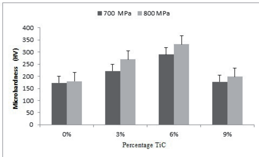
Figure 7. Microhardness in compacted sintered at 700 and 800 MPa.
