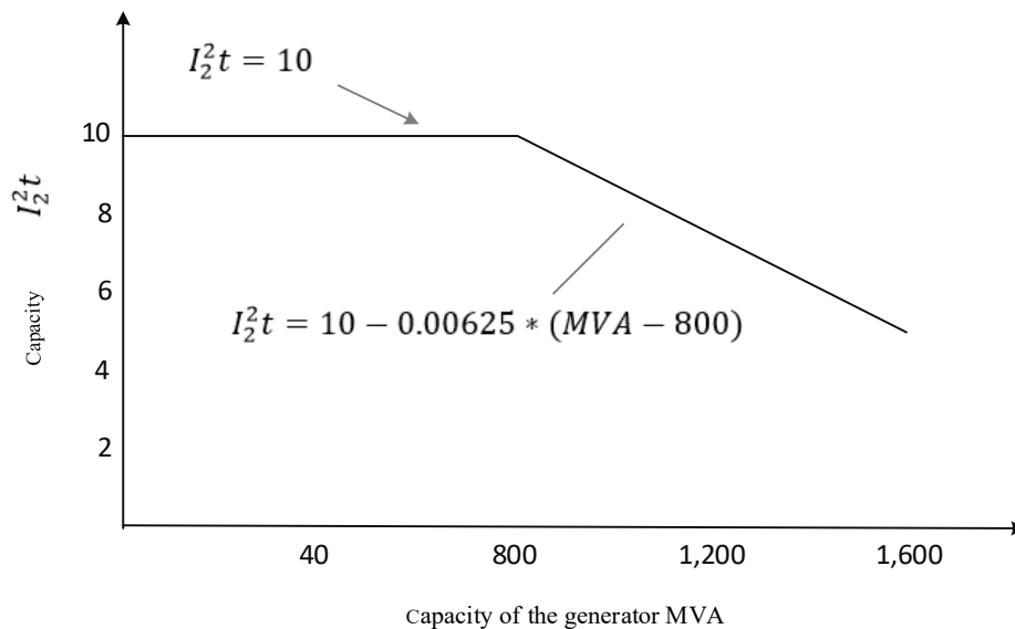
Figure 3. Current capacity of short-time imbalance in directly cooled cylindrical rotor generator (1)
