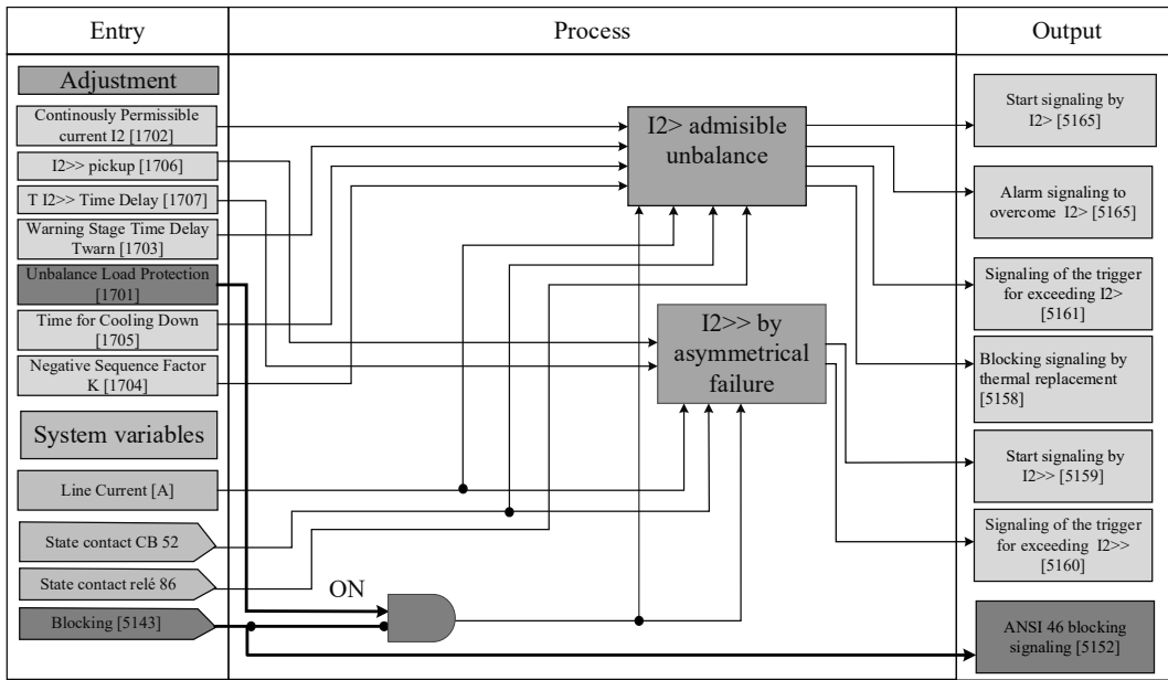
Figure 7. Confirmation sub-process ON ANSI 46 PDF (5)
