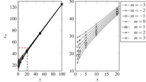
Figure 3. Upper limit, x_\infty for the integral p_m , calculated from i_\infty in Eq. (13). The right plot is a zoom of the area in the red rectangle. Results are shown for different m values
