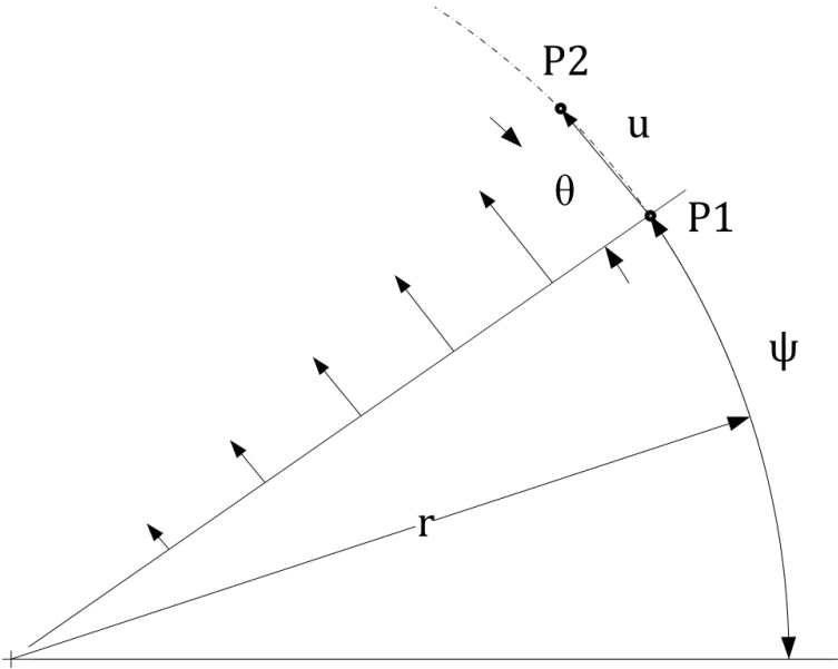
FIGURE 3. DISPLACEMENT U FROM P1(r, \psi, z) TO P2(r, \psi + \theta, z) .
