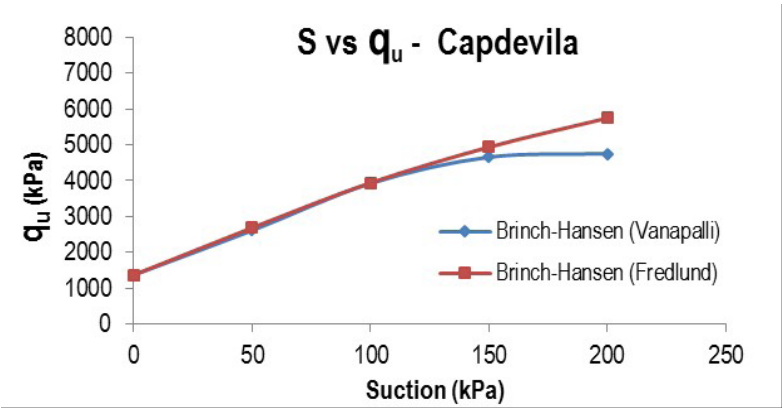
Figure 5. Curve of ultimate bearing capacity vs suction for formulating Brinch-Hansen modified of ( C_{\text{Vanapalli}} and \phi_{\text{Vanapalli}} ) and ( C_{\text{Fredlund}} and \phi_{\text{Fredlund}} ), soil - Capdevila.
