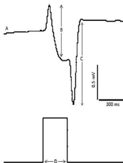
Figure 1. Electrophoretogram (ERG) response in wild untrained adults of Lucilia sericata from Colombia. Upper trace: Biphasic male ERG response showing changes in voltage: (A) Resting potential. (B) “On-response” and (C) “Off-response”. Lower trace: Characteristics of the stimulus in amplitude and duration (D).
