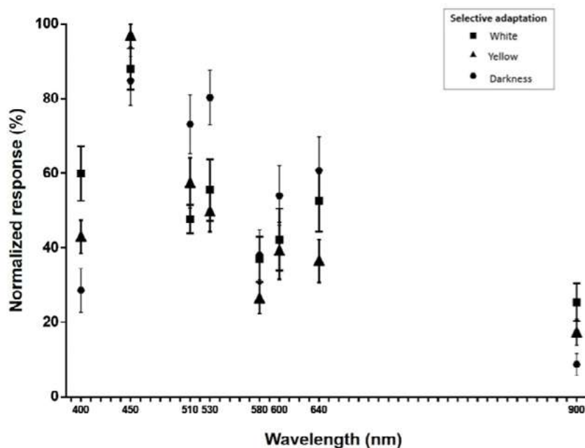
Figure 3. Whole-eye ERG threshold response curves obtained from wild untrained Lucilia sericata from Colombia. Values of the normalized “on-response” obtained after stimulation with the different wavelengths tested and with flies adapted to darkness (dots), yellow (triangles), or white (squares) lights.
