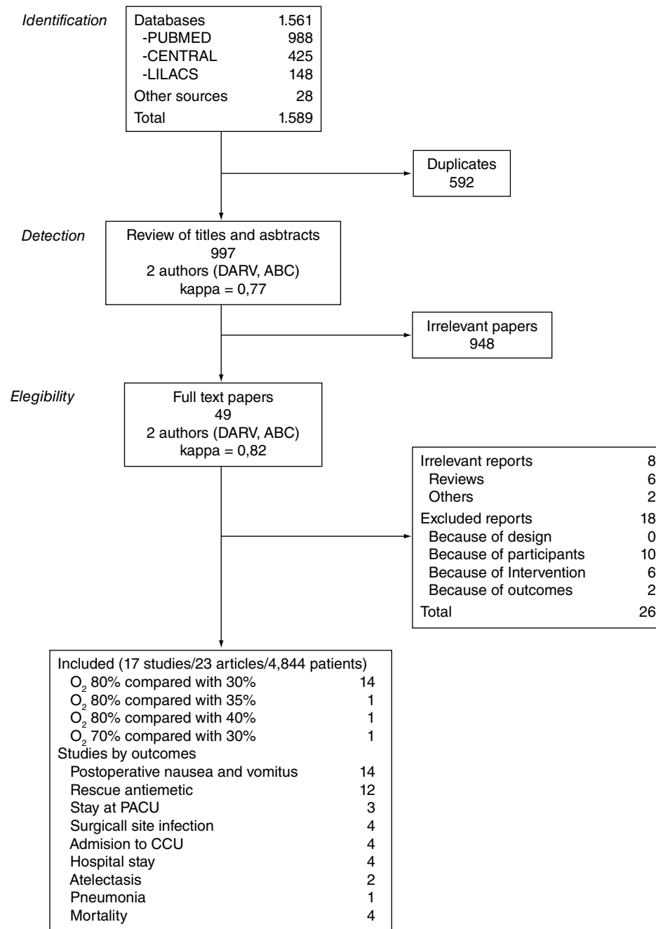
Fig. 1 – Selection Process.
