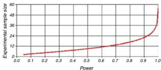
Fig. 2 – Sample size versus power graph for the study.
