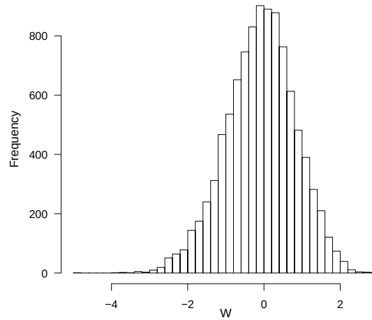
FIGURE 1: Histogram of W for m = n = 500 .
