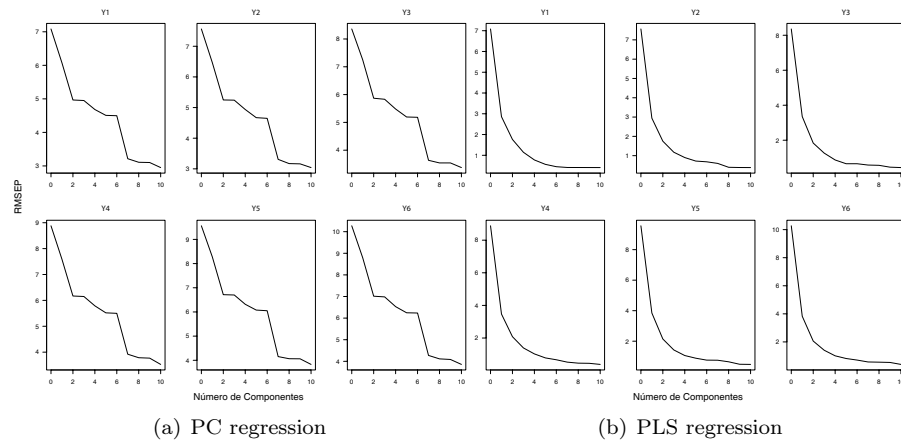
FIGURE 3: RMSEP versus number of components by PC regression and PLS regression, 2.
