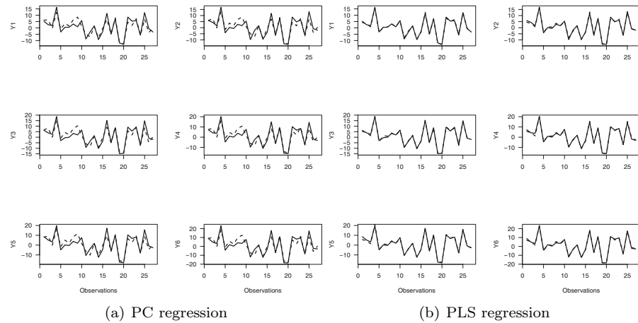
FIGURE 4: Predicted values with the observables values by PC regression and PLS regression, 2. Solid lines: Observed, dashed lines: Predicted.
