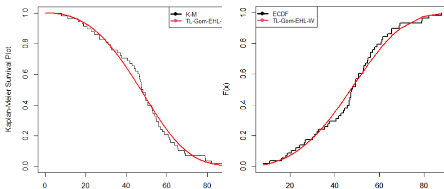
FIGURE 21: Fitted K-M survival and ECDF plots for Unemployment Insurance Data
