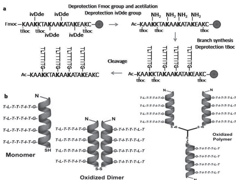
Figure 2. a. Schematic representation of the peptide synthesis. The backbone of the polypeptide was successively synthesized on TGR resin, then the Fmoc protecting group of K 1 was removed and the free amide group was acetylated. The \epsilon -amino ivDde protective groups of K 4 , K 8 , K 11 and K 15 residues were then removed so synthesis of the branches could begin. Upon completion of branch synthesis the branch C-terminal amide groups were removed in addition to the remaining backbone amino acids' protective groups. The polypeptide was cleaved from the resin by treatment with TFA/TIS/EDT/H 2 O. The steps requiring most attention were the deprotection of the K 4 , K 8 , K 11 and K 15 residues and the later coupling of the first residue of each branch. b. Schematic representation of the monomer, oxidized dimer and oxidized polymer comprised of three pennant-type monomers and a cascade-type dendrimer hub.
