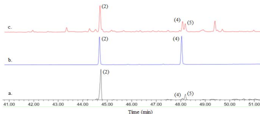
Figure 3. GC-EIMS analysis for : a. Dolabellatrienone ( 2 ) after prolonged storage; b. E. asperula extract; Fraction hexane:ethyl acetate 7:3 from E. laciniata .
