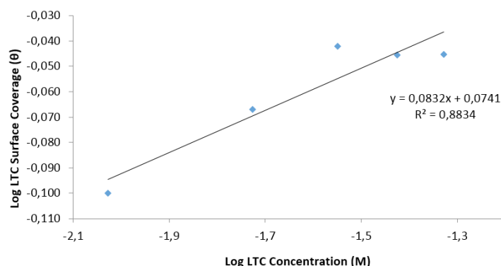
Figure 6. Freundlich isotherm plot of \log LTC surface coverage versus \log LTC concentration in 1 M \text{H}_2\text{SO}_4 .
