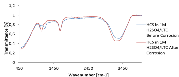
Figure 7. ATF-FTIR spectra of 1 M \text{H}_2\text{SO}_4 /LTC solution before and after HCS corrosion.
