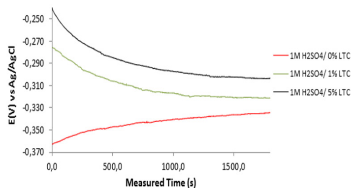
Figure 3. Variation of corrosion potential versus measured time for HCS specimen immersed in 1 M H 2 SO 4 /0%, 1% and 5% LTC.
