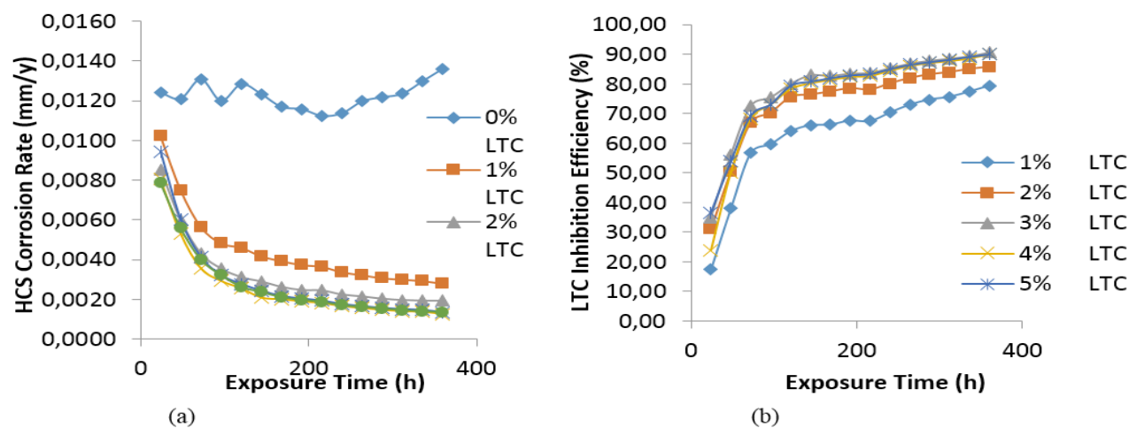
Figure 8. Plot of (a) HCS corrosion rate versus exposure time in 1 M H 2 SO 4 (b) LTC inhibition efficiency versus exposure time in 1 M H 2 SO 4 .
