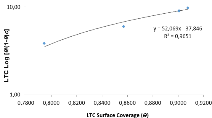
Figure 5. Frumkin isotherm plot of \log \left[ \frac{\theta}{(1-\theta)c_{\text{LTC}}} \right] versus surface coverage ( \theta ) in 1 M \text{H}_2\text{SO}_4 .
