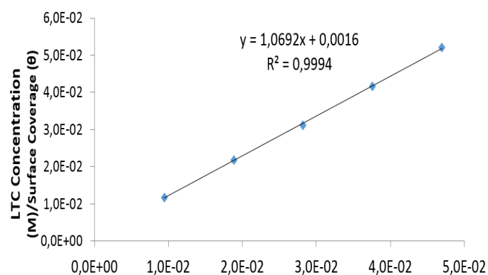
Figure 4. Langmuir isotherm plot of \frac{C_{LTC}}{\theta} versus LTC concentration in 1 M H 2 SO 4 .
