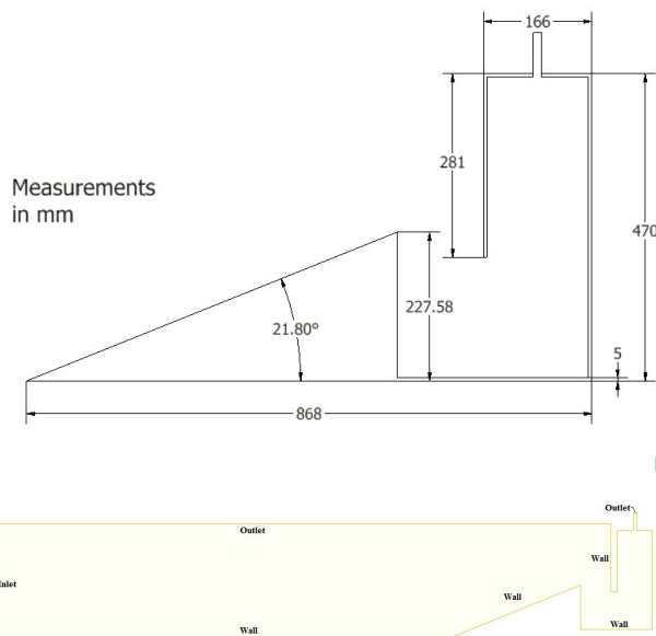
Figure 5 Wave channel for Pacific Ocean conditions
