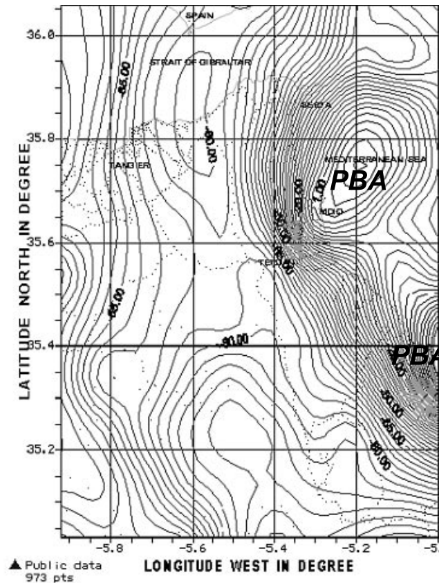
Figure 4 Bouguer anomaly map of the area of Tangier-Tetuan (interval contour 3 mGal, PBA for positive Bouguer anomalies)
