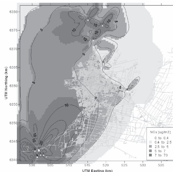
Figure 5 Average daily concentration of \text{NO}_x calculated using CALPUFF. White triangles represent the main industrial sources
