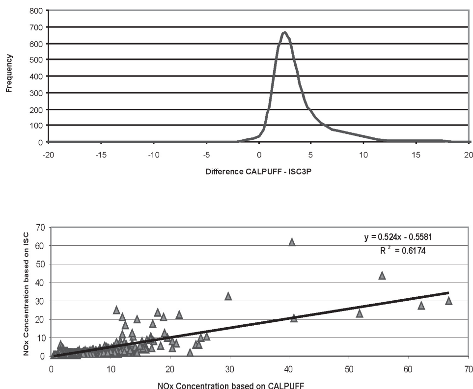
Figure 6 Comparison of the calculated \text{NO}_x concentration using ISC3P and CALPUFF. Above: Frequency distribution of the differences for all receptors. Below: Dispersion plot of the calculated concentrations
