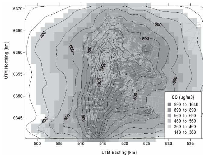
Figure 9 Calculated hourly mean values for \text{CO} ( \text{ug}/\text{m}^3 ) including all sources for Mendoza Metropolitan Area using CALPUFF
