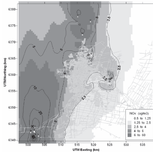
Figure 4 Average daily concentration of \text{NO}_x calculated using ISC3P. White triangles represent the main industrial sources
