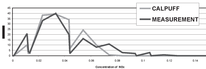
Figure 8 Comparison between calculated and measured \text{NO}_x daily mean values for year 1996
