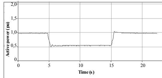
Figure 21 System response due to variation on the power load. Terminal active power at synchronous generator with neural based PSS
