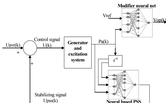
Figure 8 Basic scheme used to obtain the new training data, used to finally set up the neural based PSS.
