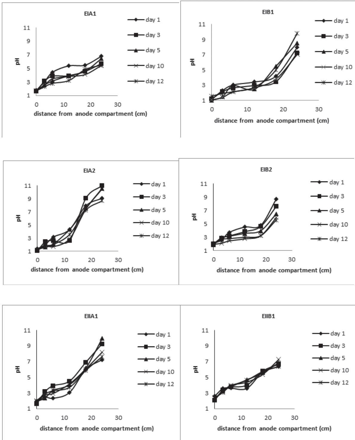
Figure 1 pH distribution during the electrokinetic experiments
