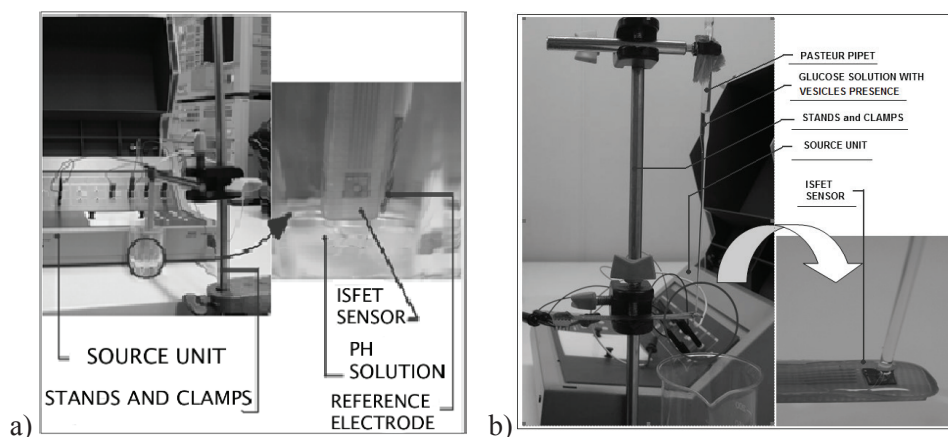
Figure 2 The experimental set-up for charge detection experiments. a) The experimental set-up for the pH – measurements. b) The experimental set-up for the vesicle detection. Both configurations guarantee the full exposure of the channel area either to the buffer or to the lipid vesicles solution
