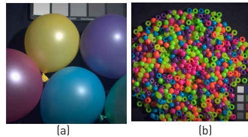
Figure 9 The RGB images mapped versions of the selected data cubes (a) Balloons and (b) Beads
