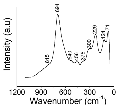
Figure 4 Raman spectra for the Nb_2O_5/H_2O_2 synthesized
