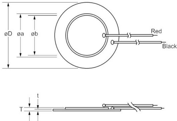
Figure 1 Murata piezoelectric illustration [16]
