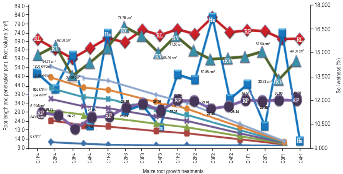
Figure 8. Root length (RL), root penetration (RP), root volume (RV) and soil wetness (Hu) versus treatment and soil wetness; shear tension ( \tau ) and normal load ( \sigma ) effects.
